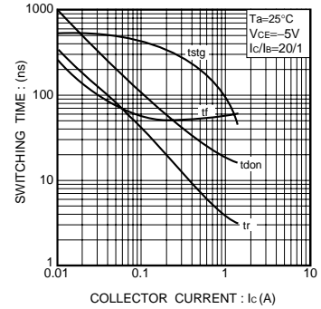
Fig.6 Switching time
