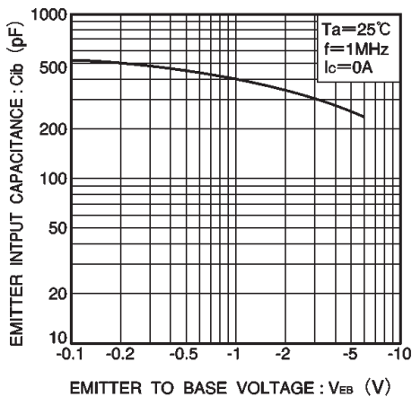
Fig.13 Emitter input capacitance vs. emitter-base voltage
