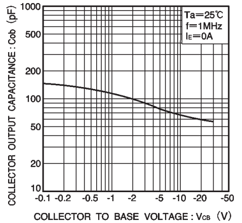
Fig.12 Collector output capacitance vs. collector-base voltage
