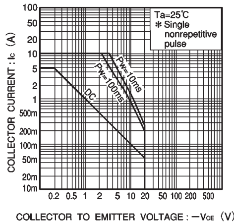
Fig.14 Safe operation area (2SB1412)
