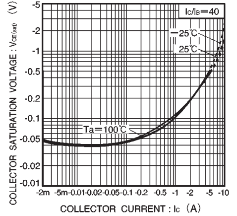
Fig.9 Collector-emitter saturation voltage vs. collector current ( IV )
