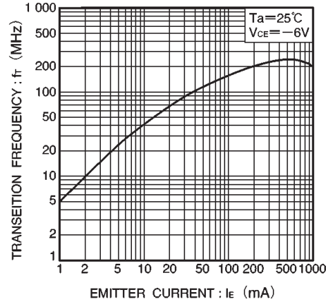
Fig.11 Gain bandwidth product vs. emitter current
