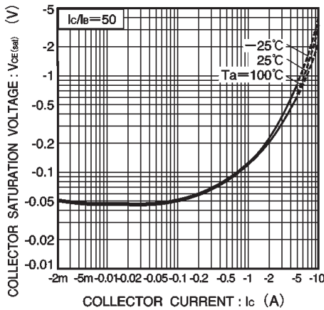
Fig.10 Collector-emitter saturation voltage vs. collector current ( V )
