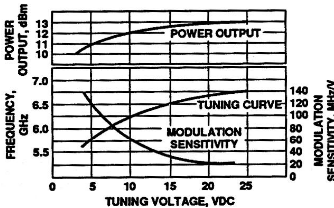
Figure 9. VTO-8580 Power Output, Frequency and Modulation Sensitivity vs. Tuning Voltage.
