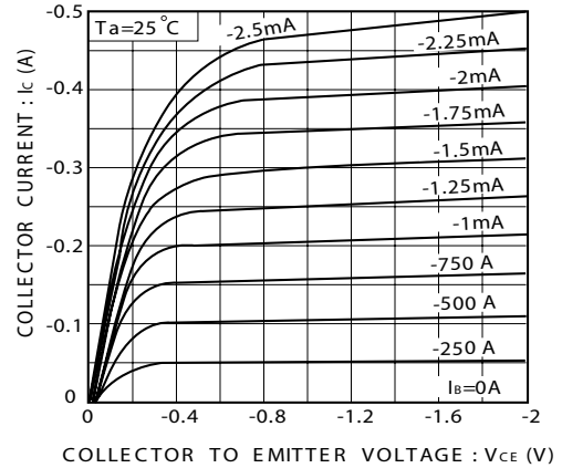
FIG.2 Grounded emitter output characteristics
