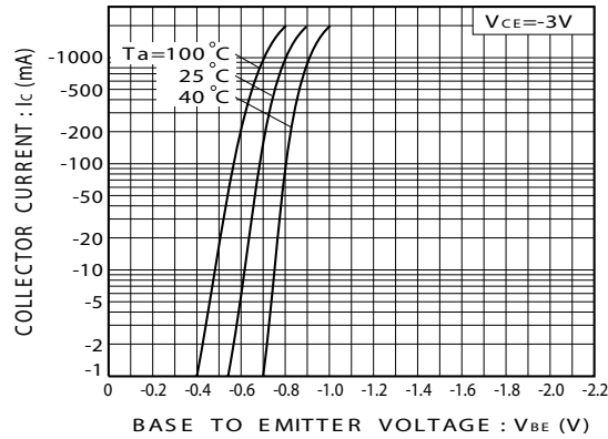
FIG.1 Grounded emitter propagation characteristics
