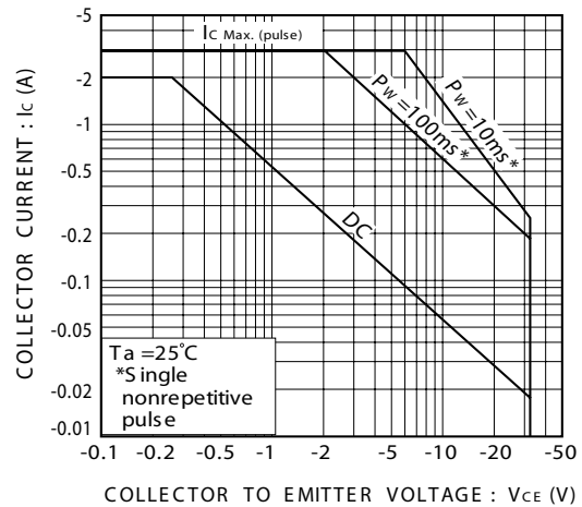
FIG.10 Safe operation area
