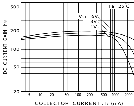
FIG.3 DC current gain vs. collector current
