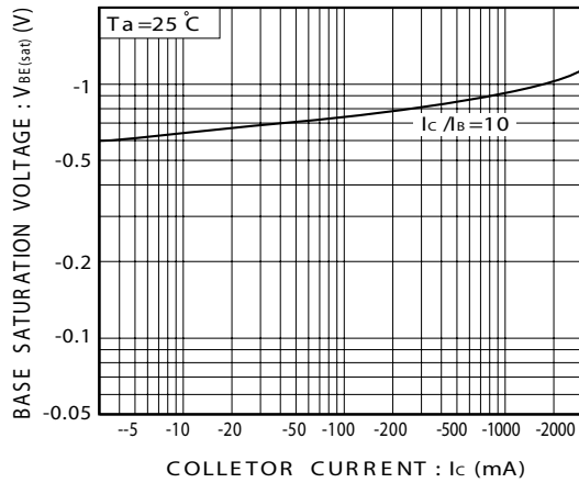
FIG.7 Base-emitter saturation voltage vs. collector current
