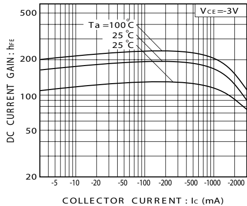
FIG.4 DC current gain vs. collector current
