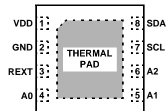
ISL29002 (8 LD ODFN) TOP VIEW
