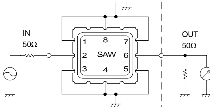
Fig.1 Measuring circuit
