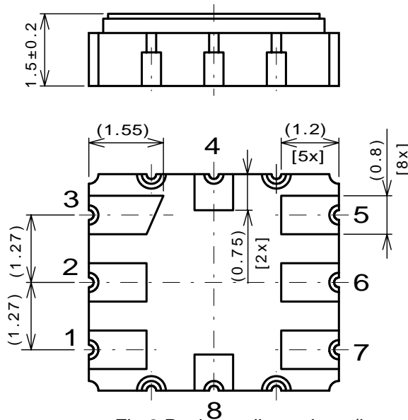
Fig.2 Package dimensions (in mm)
