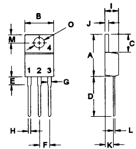
TO-220
