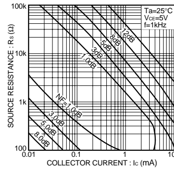
Fig.18 Noise characteristics ( III )
