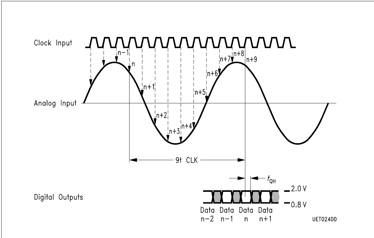
Figure 6 Diagram of Complete Timing
