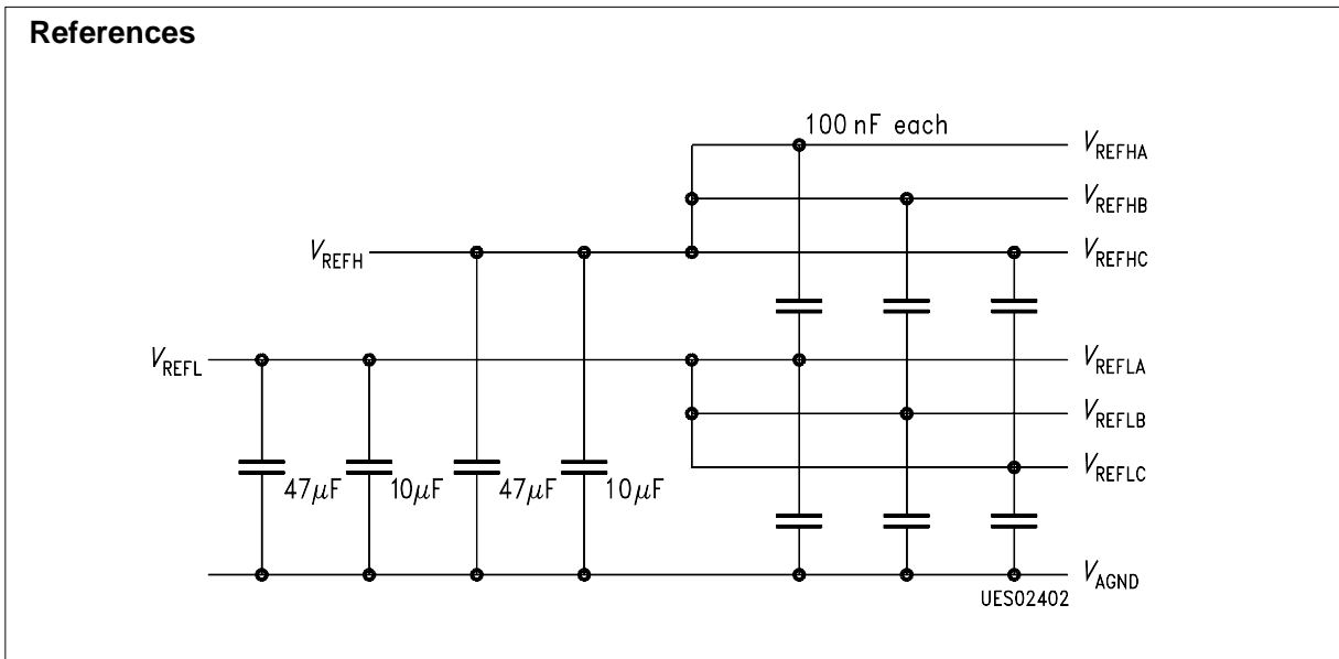
Figure 8 Blocking the SDA 9205-2
