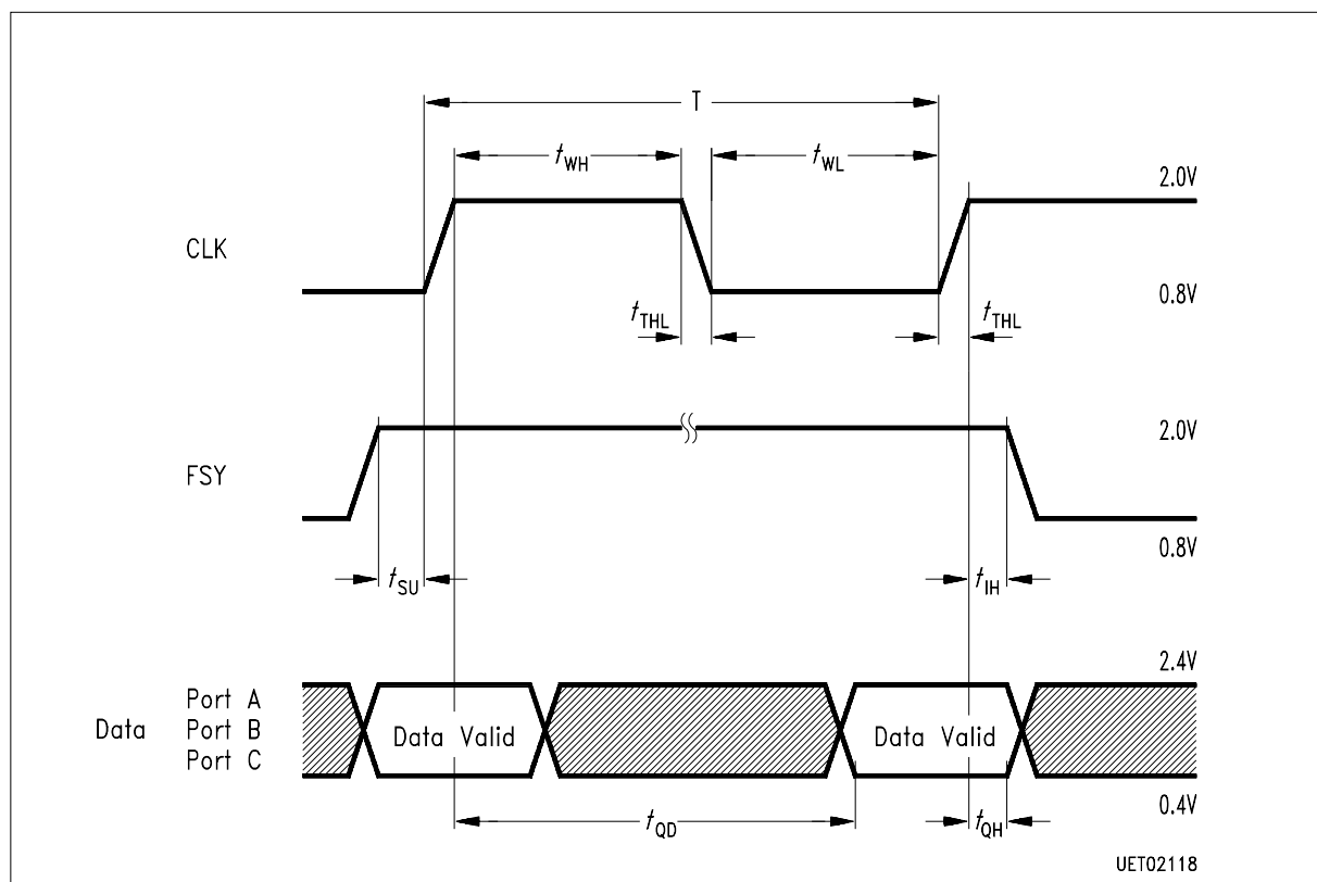
Figure 5 Timing Diagram Port A, B, C
