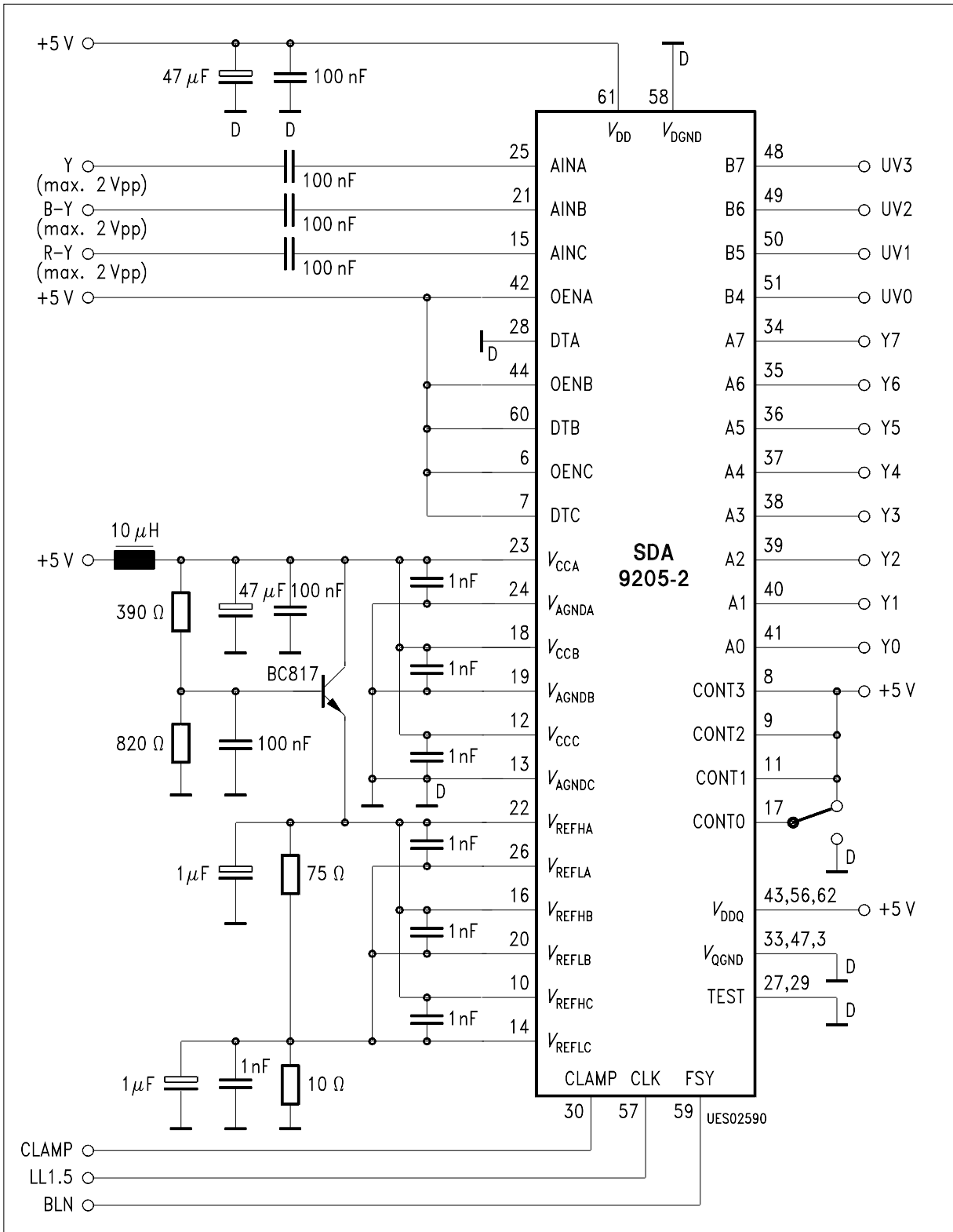
Figure 9 Application Circuit 1 (4:1:1 Format, for Siemens Featurebox)
