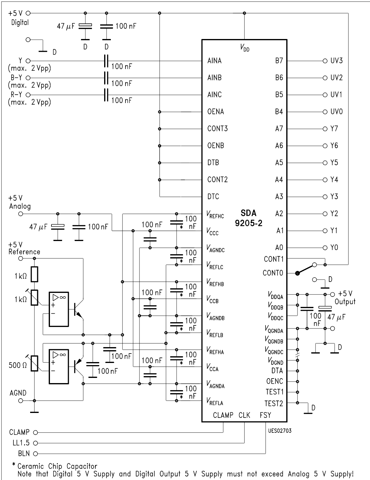
Figure 10 Application Circuit 2 (4:1:1 Format, for General Application)
