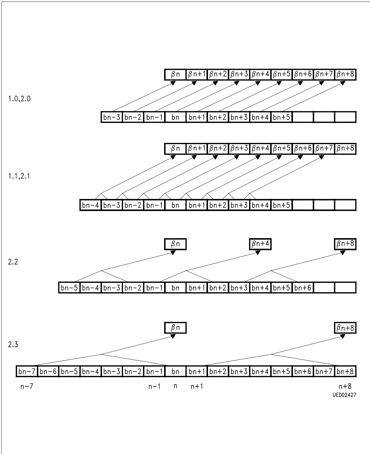
Figure 3 DSP Function
