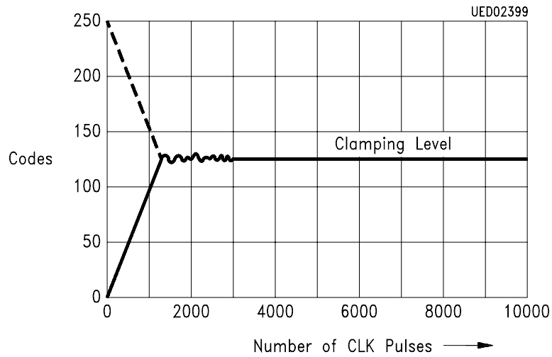
Figure 1 Typical Clamp Timing Diagram
