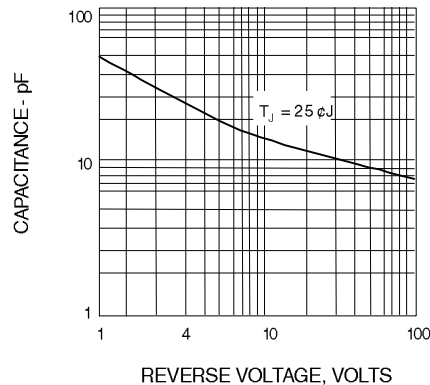
Fig. 4-TYPICAL JUNCTION CAPACITANCE
