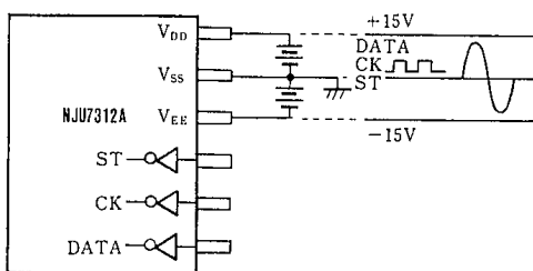
Dual Power Supply (+ and -)
