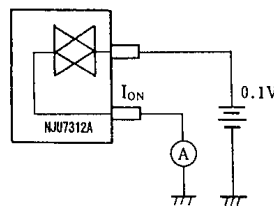
( Circ.2 )
