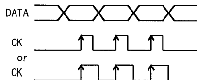
(Timing Chart)
