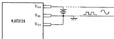
Single Power Supply (+)
