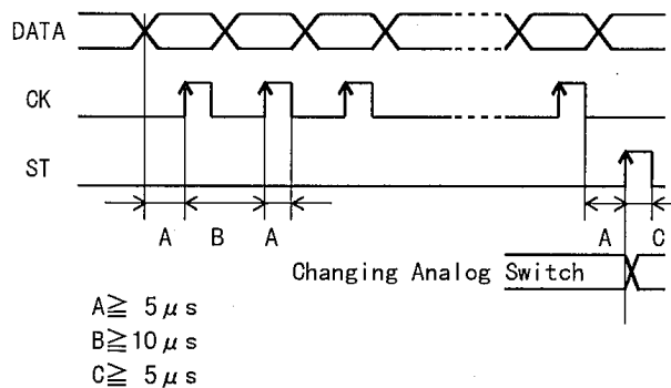
(Detailed Timing)
