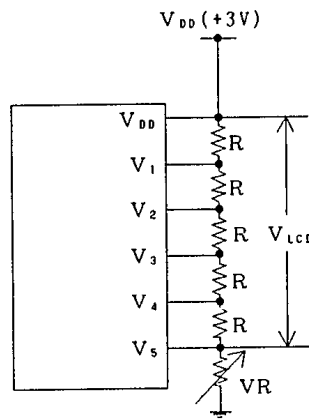
(a) 1/5 Bias (1/18 Duty)
