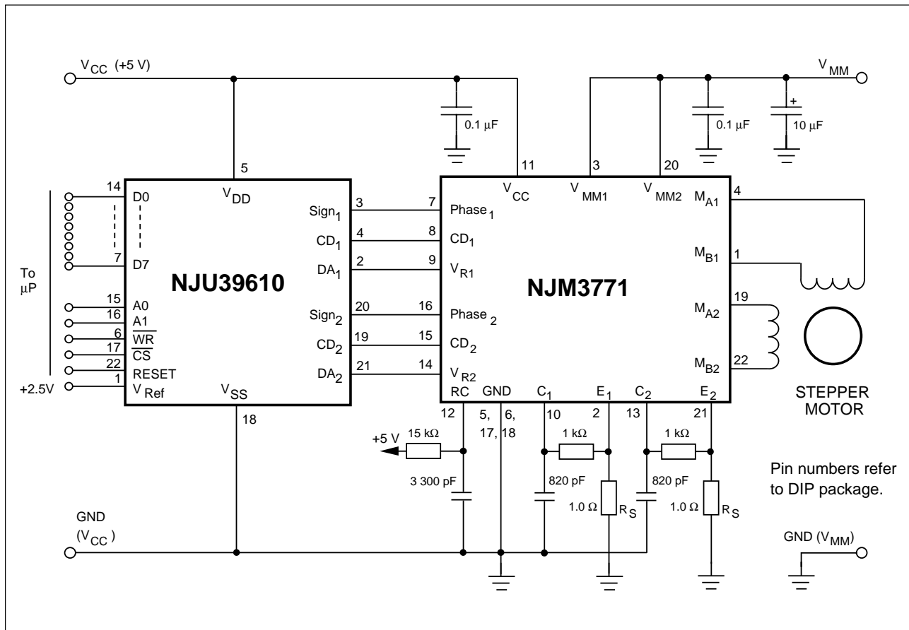
Figure 14. Typical application in a microprocessor based system.
