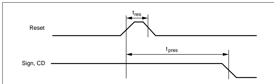
Figure 12. Timing of Reset
