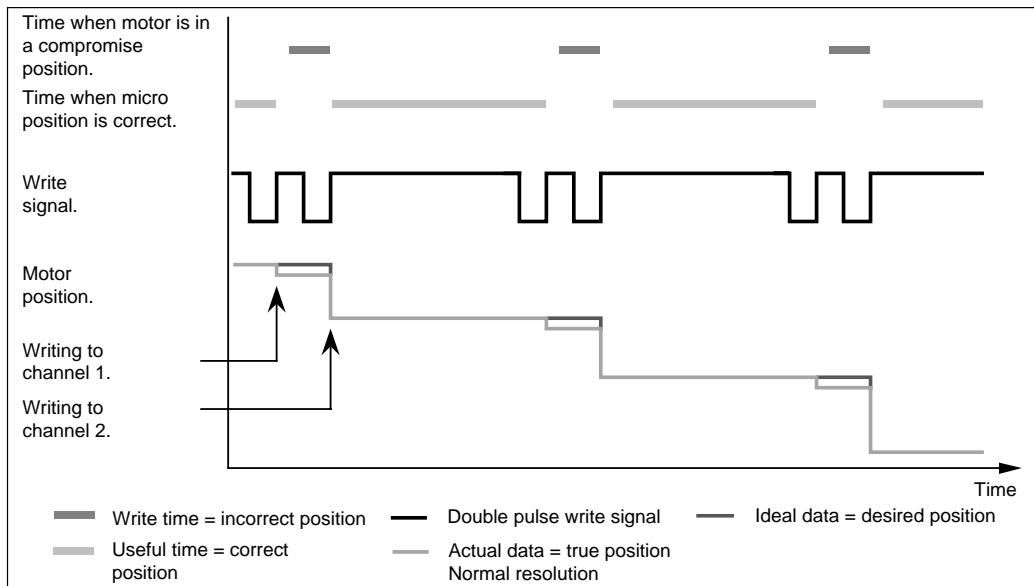
Figure 9. Double pulse programming, in- and output signals.
