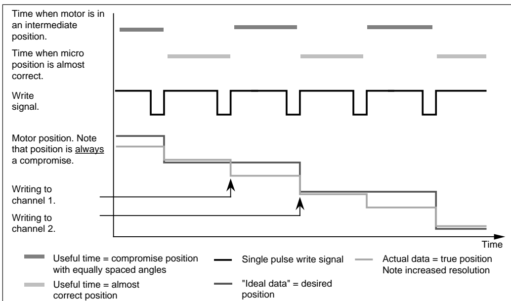
Figure 10. Single pulse programming, in- and output signals.
