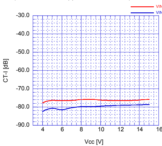
Crosstalk vs. Supply Voltage (Vin=4.43MHz 1Vpp Vin4 to Vin1,2,3)
