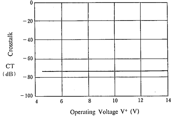
Crosstalk(IN2A to OUT2)vs. Operating Voltage ( T_a = 25^\circ\text{C} )
