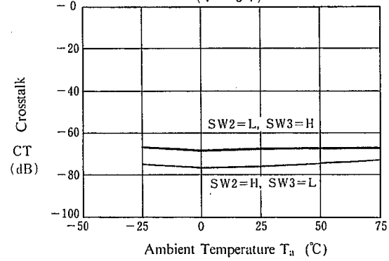
Crosstalk(IN1B to OUT1)vs. Ambient Temperature ( V^+ = 5\text{V} )
