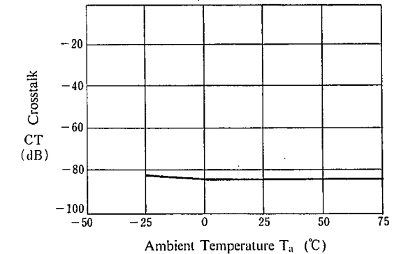
Crosstalk(IN1B to OUT1)vs. Ambient Temperature ( V^+ = 5\text{V} )
