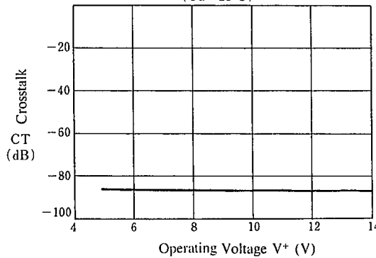
Crosstalk(IN1B to OUT1)vs. Operating Voltage ( T_a = 25^\circ\text{C} )
