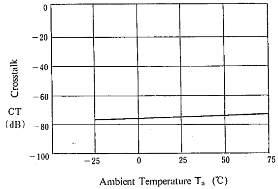
Crosstalk(IN2A to OUT2)vs. Ambient Temperature ( V^+ = 5\text{V} )
