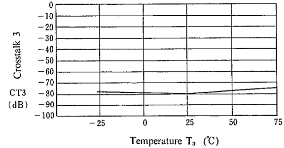
Crosstalk 3 vs. Temperature
