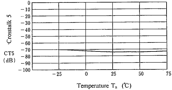
Crosstalk 5 vs. Temperature
