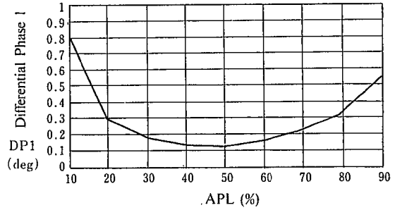
Differential Phase 1 vs. APL ( T_a = 25^\circ\text{C} )
