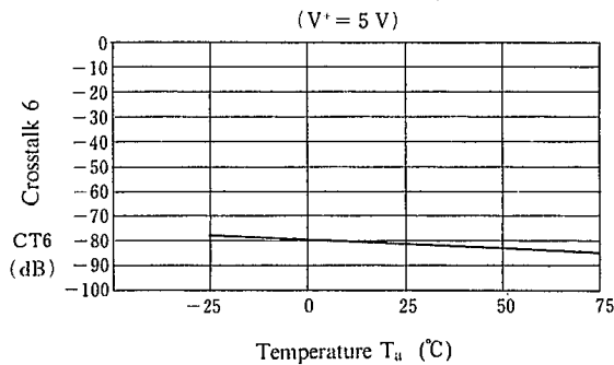
Crosstalk 6 vs. Temperature
