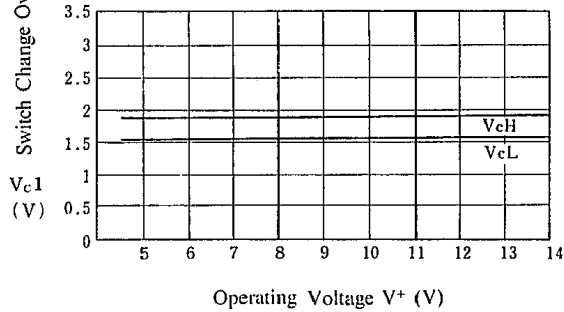
Switch Change Over 1 vs. Operating Voltage
