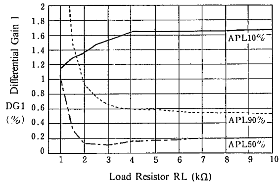
Differential Gain 1 vs. Load Resistor
