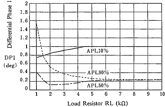
Differential Phase 1 vs. Load Resistor
