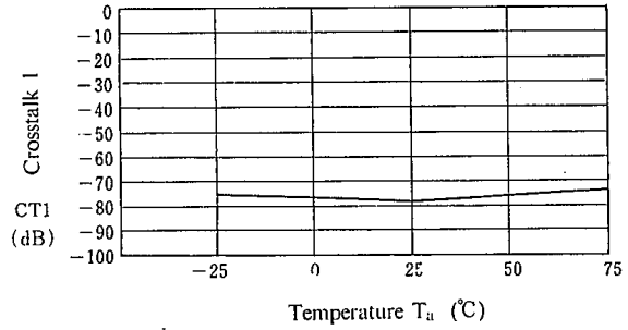
Crosstalk 1 vs. Temperature
