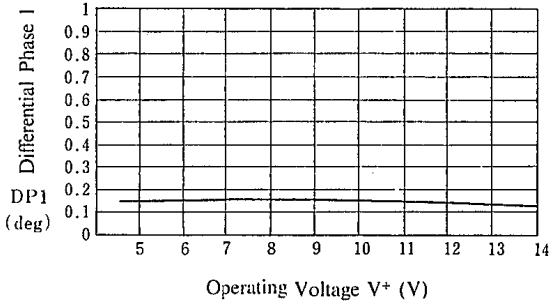
Differential Phase 1 vs. Operating Voltage
