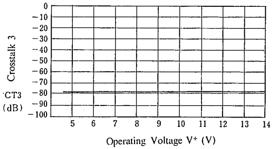
Crosstalk 3 vs. Operating Voltage
