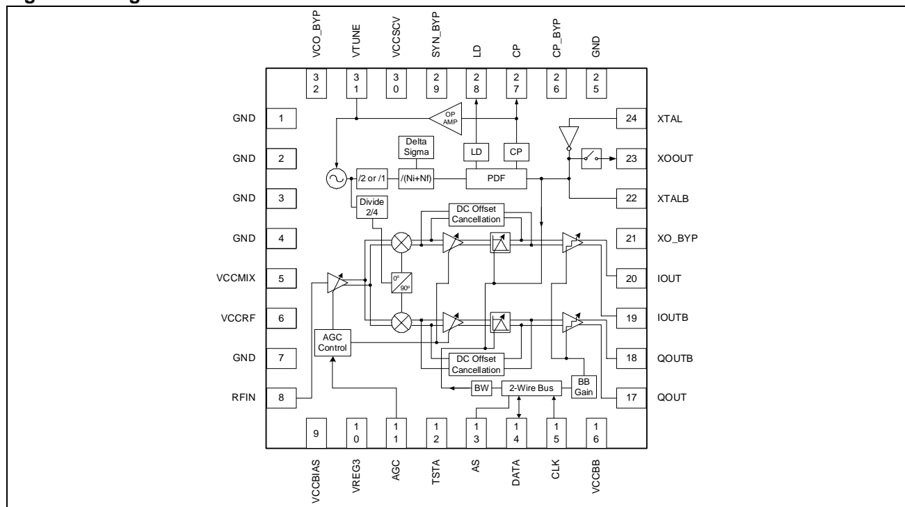
Figure 2. Integrated silicon tuner
