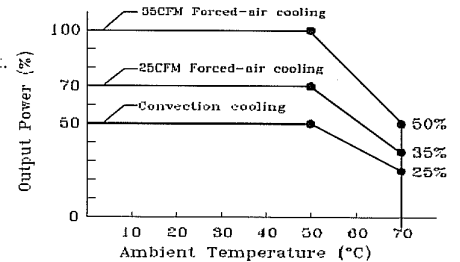
DERATING CURVE
