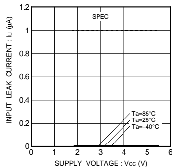
Fig.21 Input leakage current I IL (A0,A1,A2,SCL,WP)
