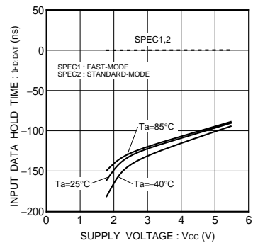
Fig.34 Input data hold time t HD,DAT(LOW)
