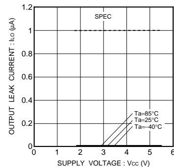
Fig.22 Output leakage current I LO (SDA)
