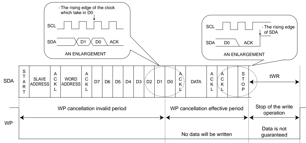
Fig.13 WP EFFECTIVE TIMING
