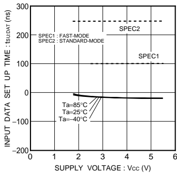
Fig.35 Input data setup time t_{SU,DAT}(HIGH)
