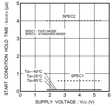
Fig.31 Start condition hold time t HD,STA
