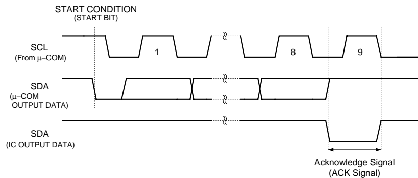
Fig.7 ACKNOWLEDGE RESPONSE FROM RECEIVER
