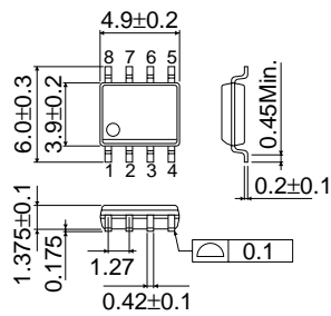
Fig.1(c) PHYSICAL DIMENSION (Units : mm) SOP-J8 (BR24L16FJ-W)
