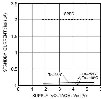
Fig.27 Standby current I bb
