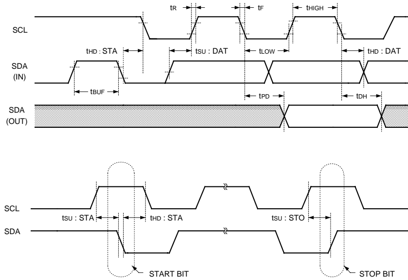
Fig.4 SYNCHRONOUS DATA TIMING
