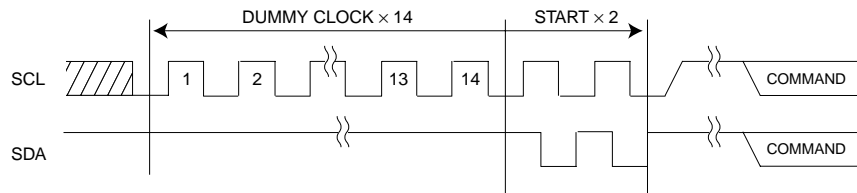
Fig.14-(a) DUMMY CLOCK × 14 + START + START
