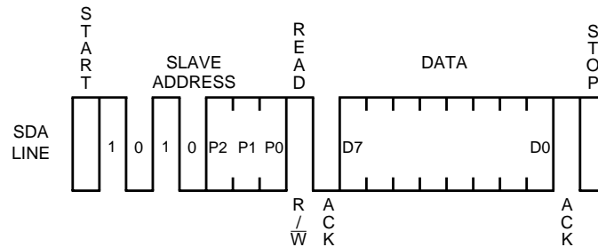
Fig.10 CURRENT READ CYCLE TIMING
