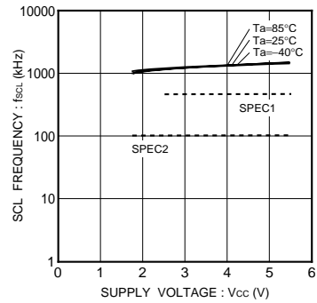
Fig.28 Clock frequency f scL
