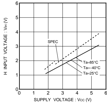
Fig.17 High input voltage V IH (A0,A1,A2,SCL,SDA,WP)
