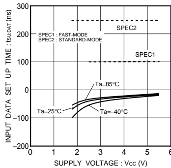
Fig.36 Input data setup time t_{SU,DAT}(LOW)
