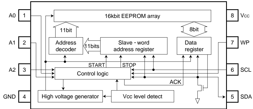
Fig.2 BLOCK DIAGRAM
