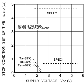
Fig.41 Stop condition setup time t_{SU,sto}
