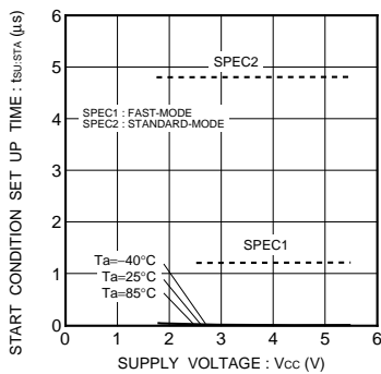
Fig.32 Start condition setup time t SU,STA
