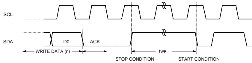
Fig.5 WRITE CYCLE TIMING
