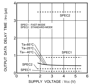
Fig.37 Output data delay time t_{p0}
