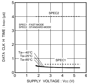
Fig.29 Data clock "H" period t HIGH
