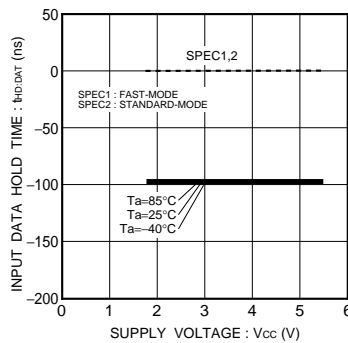
Fig.33 Input data hold time t HD,DAT(HIGH)
