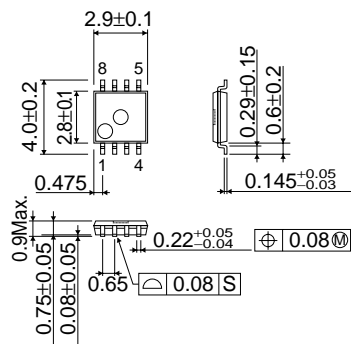
Fig.1(e) PHYSICAL DIMENSION (Units : mm) MSOP8 (BR24L16FVM-W)
