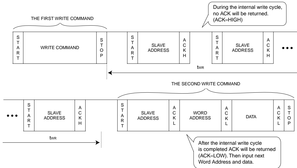
Fig.15 SUCCESSIVE WRITE OPERATION BY ACKNOWLEDGE POLLING
