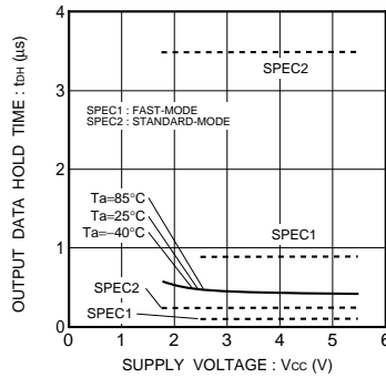
Fig.39 Output data hold time t_{dH0}
