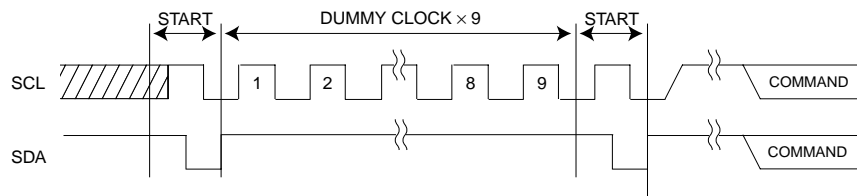
Fig.14-(b) START+ DUMMY CLOCK × 9 + START
