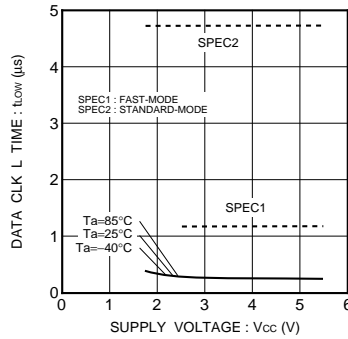
Fig.30 Data clock "L" period t LOW
