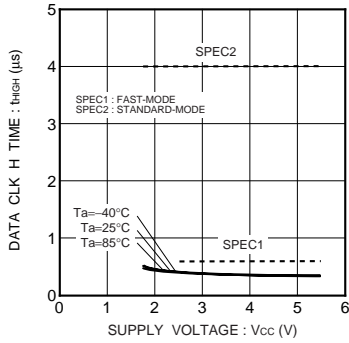
Fig.29 Data clock "H" period t HIGH
