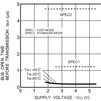
Fig.42 BUS free time tbuF
