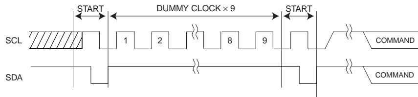
Fig.14-(b) START+ DUMMY CLOCK × 9 + START
