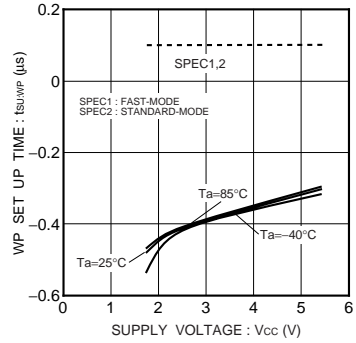
Fig.48 WP setup time t_{SU:WP}
