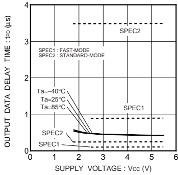
Fig.38 Output data delay time tp1
