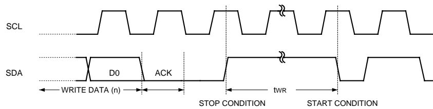
Fig.5 WRITE CYCLE TIMING
