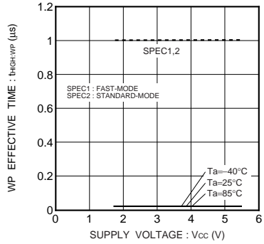
Fig.49 WP high period t_{HIGH:WP}
