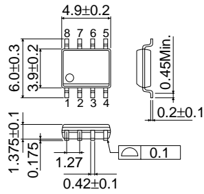
Fig.1(c) PHYSICAL DIMENSION (Units : mm) DOP-J8 (BR24L04FJ-W)
