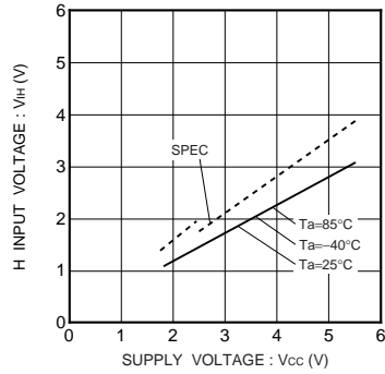
Fig.17 High input voltage V IH (A1,A2,SCL,SDA,WP)
