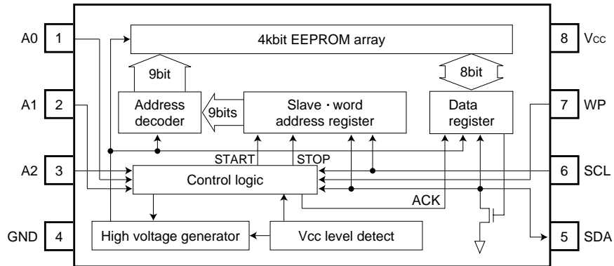
Fig.2 BLOCK DIAGRAM
