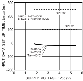
Fig.35 Input data setup time tsu:DAT(HIGH)
