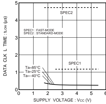
Fig.30 Data clock "L" period t LOW
