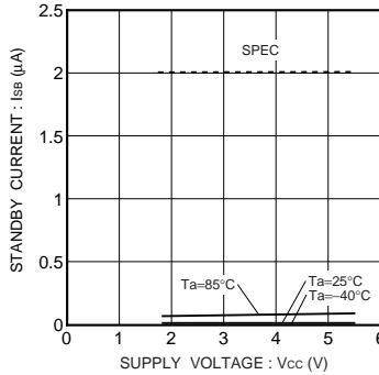
Fig.27 Standby current I BB
