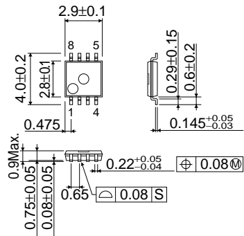
Fig.1(e) PHYSICAL DIMENSION (Units : mm) MSOP8 (BR24L04FVM-W)
