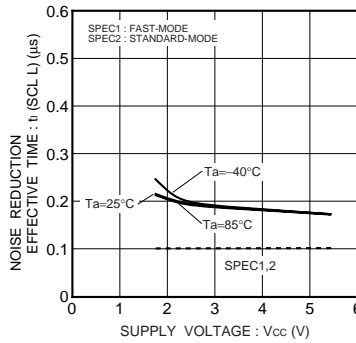
Fig.45 Noise spike width t_i (SCL L)
