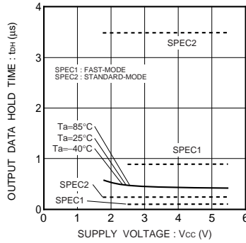
Fig.39 Output data hold time tdH0
