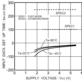
Fig.36 Input data setup time tsu:DAT(LOW)
