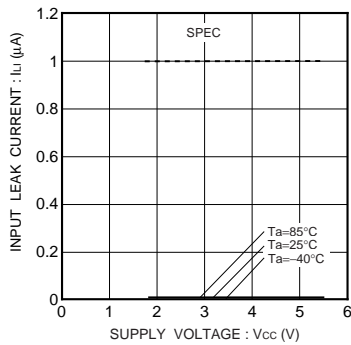
Fig.21 Input leakage current I i (A1,A2,SCL,WP)
