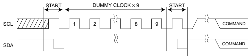
Fig.14-(b) START+ DUMMY CLOCK \times 9 + START
