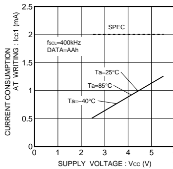
Fig.23 Write operating current I_{CC1} ( f_{SCL}=400kHz )
