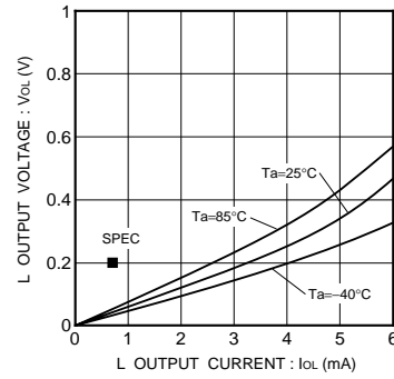
Fig.19 Low output voltage V_{OL-IOL} ( V_{CC}=1.8V )
