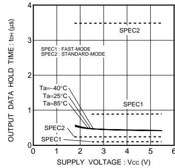
Fig.40 Output data hold time t_{dh1}
