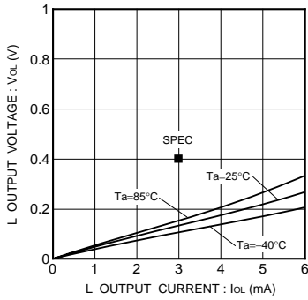
Fig.20 Low output voltage V_{OL-IOL} ( V_{CC}=2.5V )
