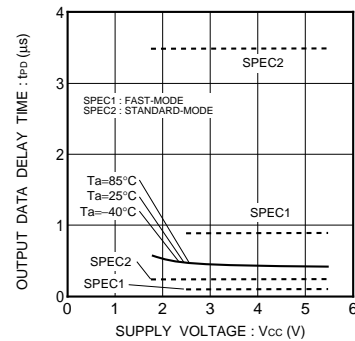
Fig.37 Output data delay time t_{pd0}
