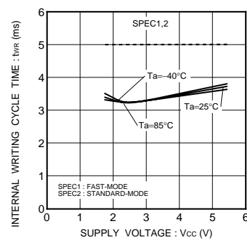
Fig.43 Write cycle time t_{wr}
