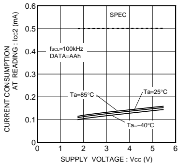
Fig.26 Read operating current I cc2 (fscl=100kHz)
