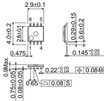
Fig.1(e) PHYSICAL DIMENSION (Units : mm) MSOP8 (BR24L01AFVM-W)
