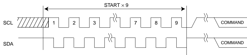
Fig.14-(c) START \times 9
