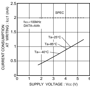
Fig.25 Write operating current I_{CC1} ( f_{SCL}=100kHz )
