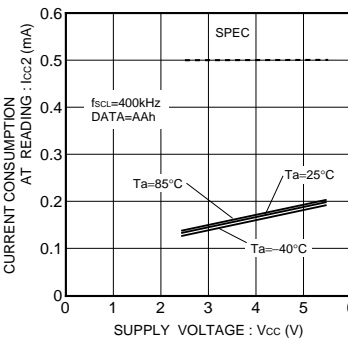
Fig.24 Read operating current I_{CC2} ( f_{SCL}=400kHz )
