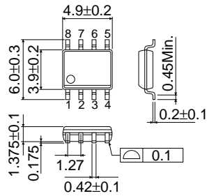
Fig.1(c) PHYSICAL DIMENSION (Units : mm) SOP-J8 (BR24L01AFJ-W)
