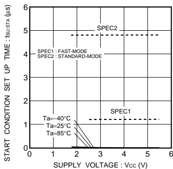
Fig.32 Start condition setup time t SU,STA
