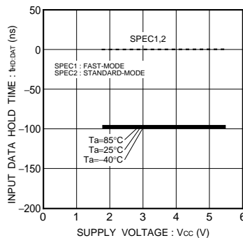
Fig.33 Input data hold time t HD,DAT(HIGH)
