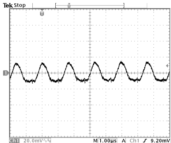
Fig.26: Output ripple and noise at 12Vin, 3.3V/8Aout
