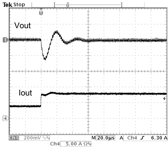
Fig.27: Output voltage response to step load change at 5A/us from 50% to 100% (12Vin, 3.3Vout)
