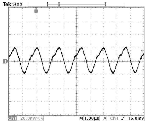
Fig.22: Output ripple and noise at 12Vin, 6.6V/8Aout
