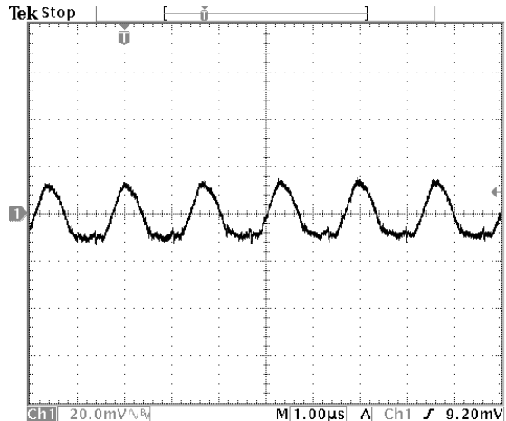
Fig.26: Output ripple and noise at 12Vin, 3.3V/8Aout
