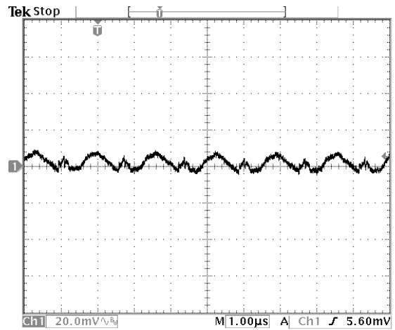
Fig.30: Output ripple and noise at 12Vin, 0.8V/8Aout
