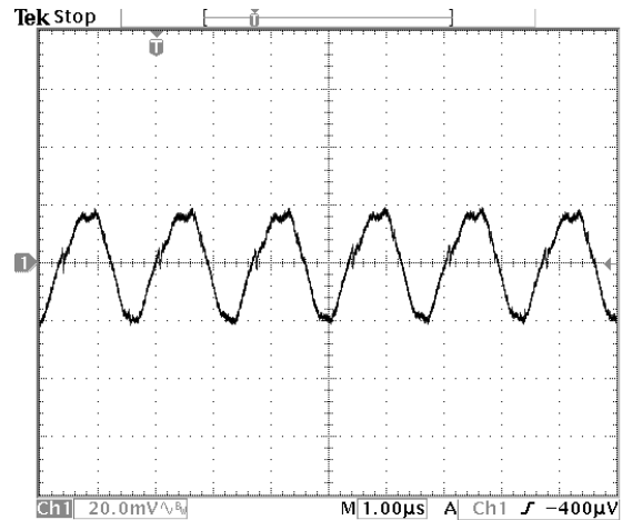
Fig.16: Output ripple and noise at 12Vin, 6.6V/6Aout
