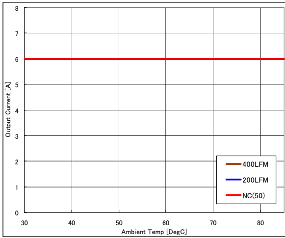
Fig.1: Output current vs. ambient temperature and air velocity at 12Vin, 0.8V to 3.3V out
