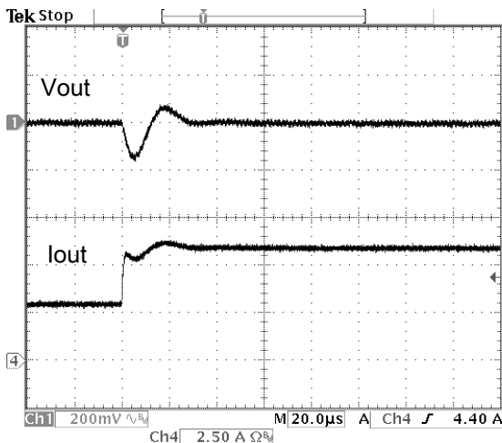
Fig.25: Output voltage response to step load change at 5A/us from 50% to 100% (12V in , 0.8V out )
