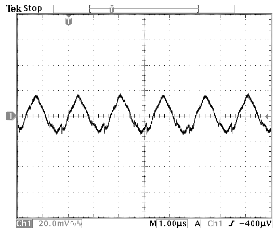
Fig.20: Output ripple and noise at 12Vin, 3.3V/6Aout
