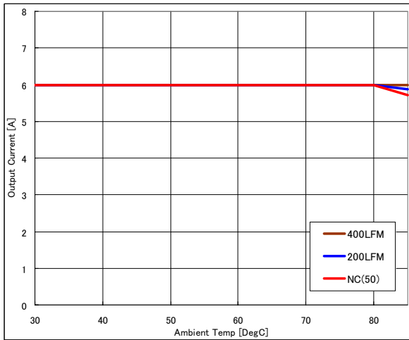
Fig.3: Output current vs. ambient temperature and air velocity at 12Vin, 6.0V out
