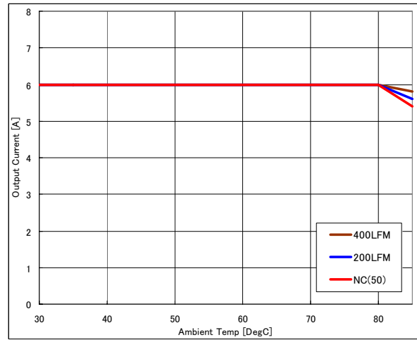
Fig.4: Output current vs. ambient temperature and air velocity at 12Vin, 6.6V out
