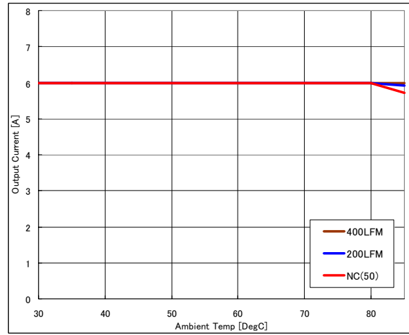
Fig.2: Output current vs. ambient temperature and air velocity at 12Vin, 5.0V out
