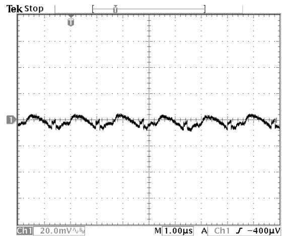
Fig.24: Output ripple and noise at 12Vin, 0.8V/6Aout
