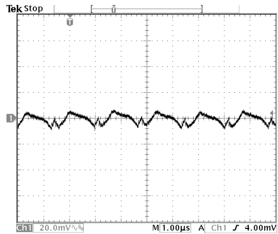
Fig.21: Output ripple and noise at 12V in , 0.8V/4A out
