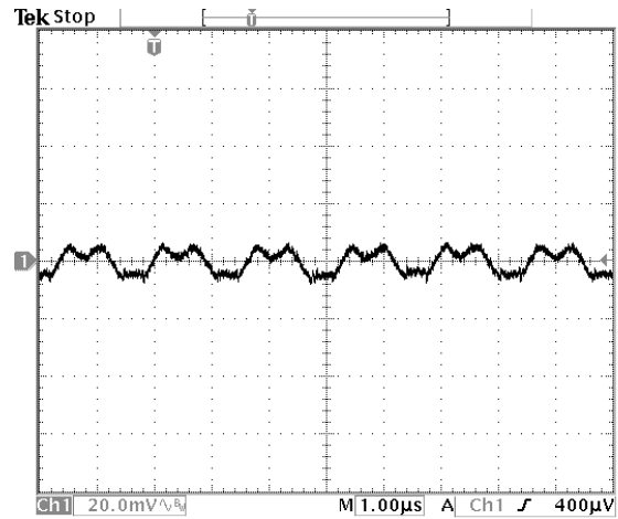
Fig.15: Output ripple and noise at 5.0Vin, 0.8V/6Aout
