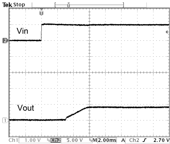
Fig.14: Turn on delay time at 5.0Vin, 0.8V/6A out
