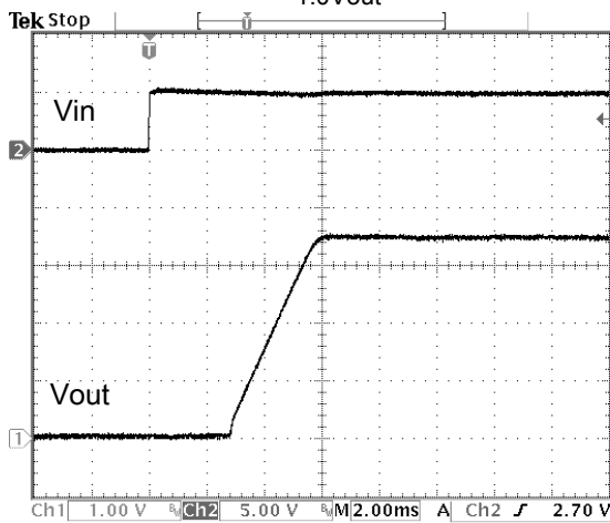
Fig.10: Turn on delay time at 5.0Vin, 3.465V/6A out
