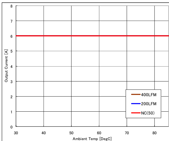
Fig.1: Output current vs. ambient temperature and air velocity at 5.0Vin, 0.8V to 3.465V out
