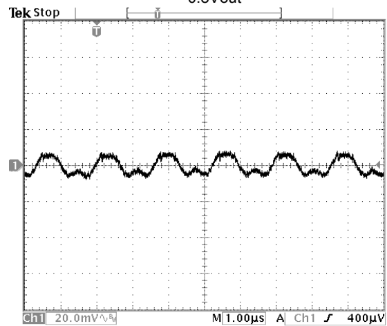
Fig.11: Output ripple and noise at 5.0Vin, 3.465V/6Aout
