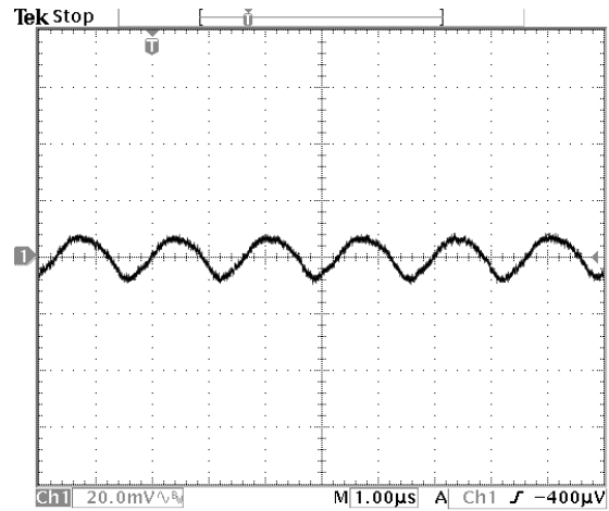
Fig.15: Output ripple and noise at 5.0Vin, 0.8V/3Aout
