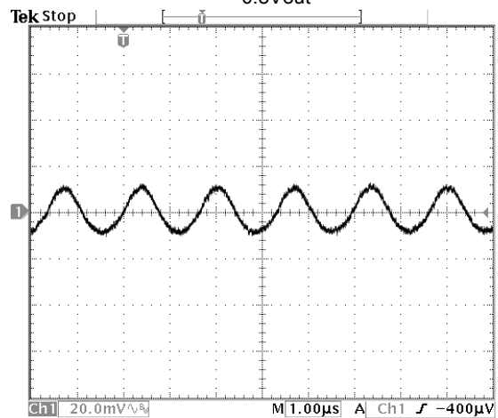
Fig.11: Output ripple and noise at 5.0Vin, 3.465V/3Aout
