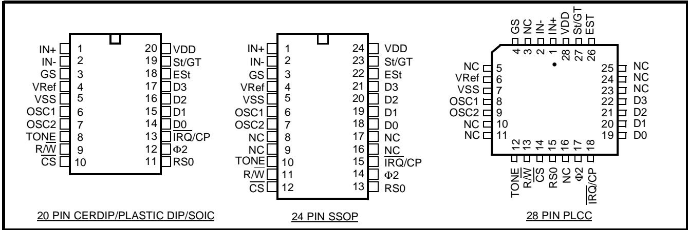
Figure 2 - Pin Connections
