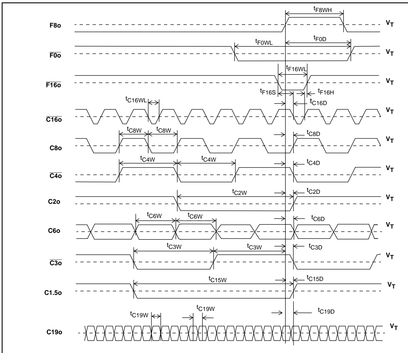
Figure 20 - Output Timing 1
