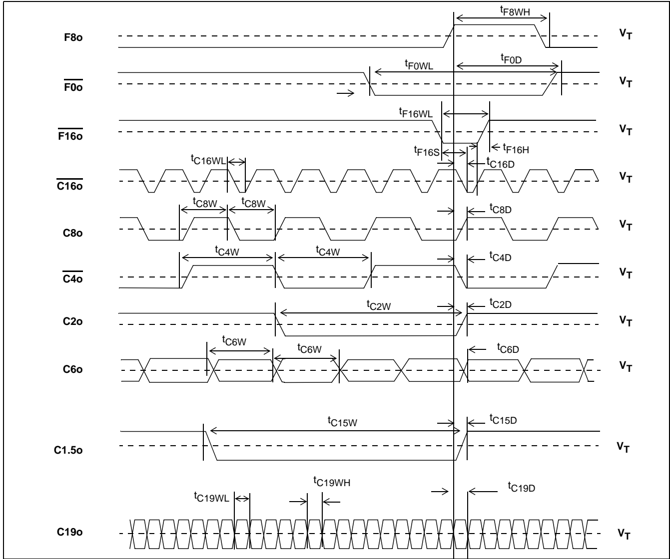
Figure 14 - Output Timing 1
