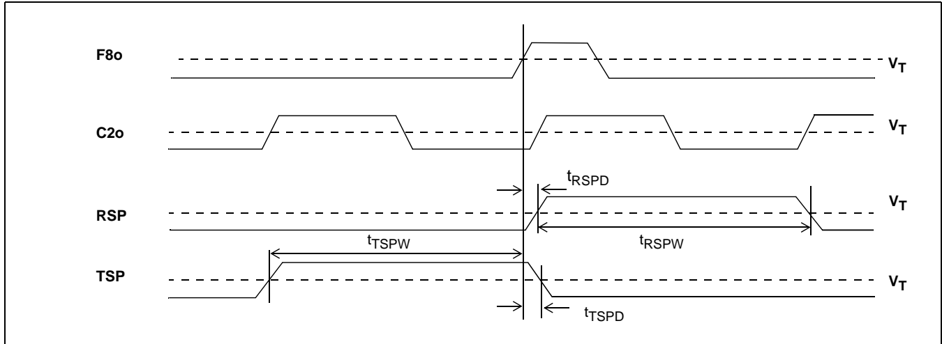
Figure 15 - Output Timing 2
