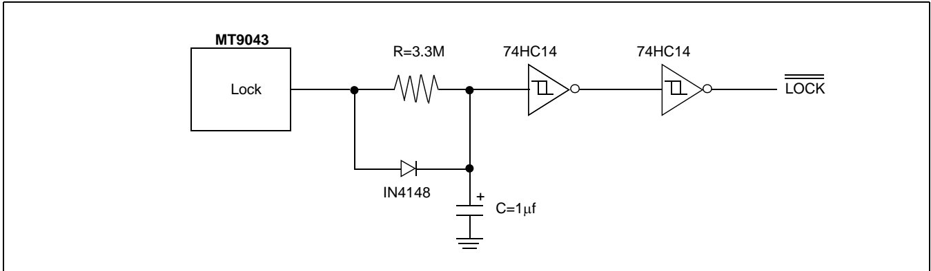
Figure 11 - Time-constant Circuit
