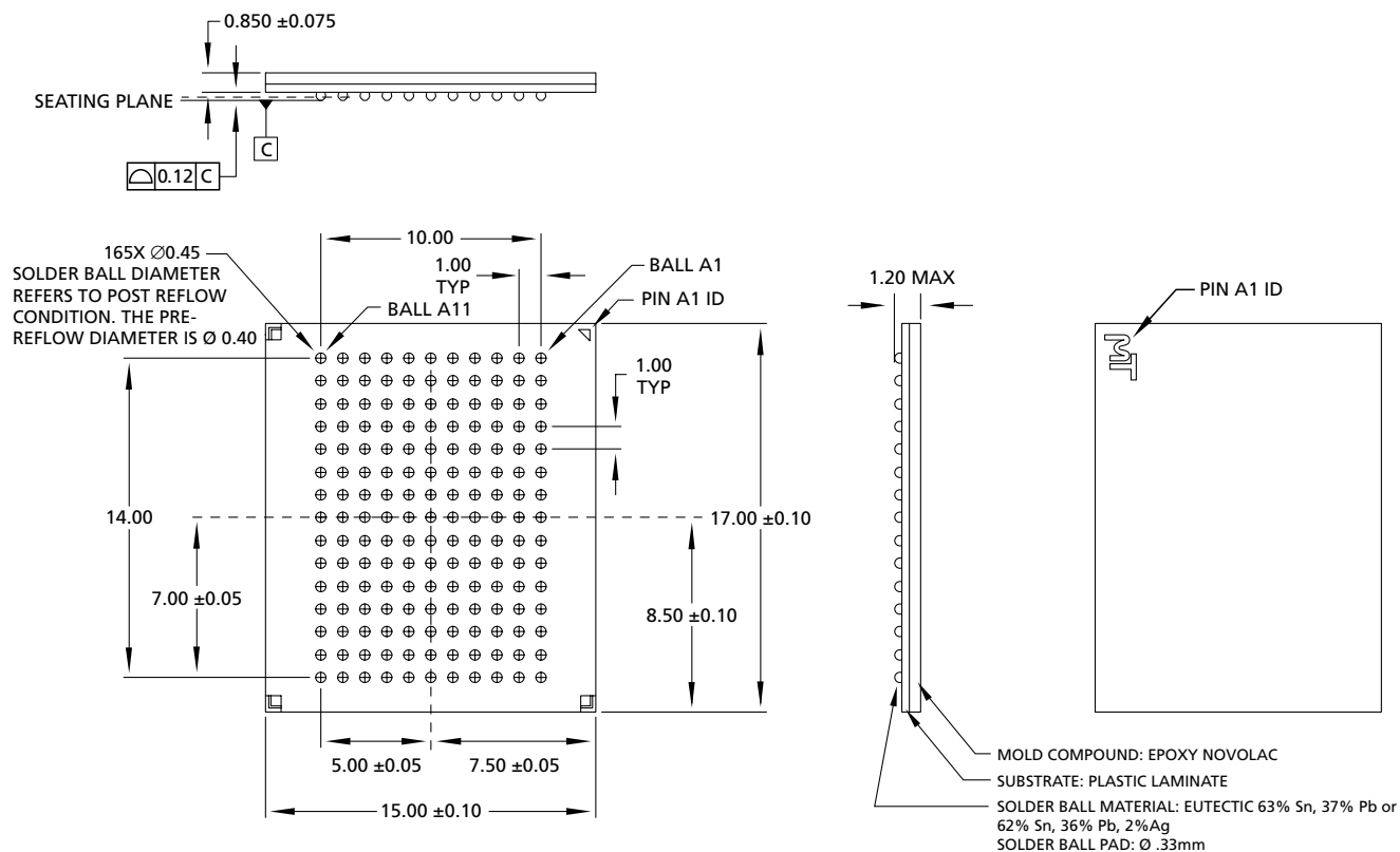
Figure 11 165-Ball FBGA
