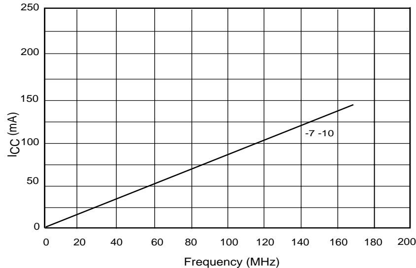
Figure 1: I_{CC} vs Frequency
