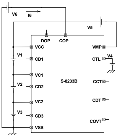
Measurement circuit 5
