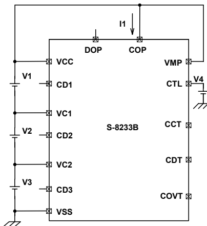
Measurement circuit 9
