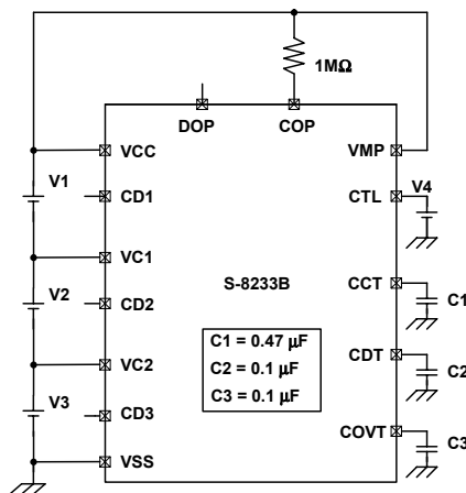
Measurement circuit 6
