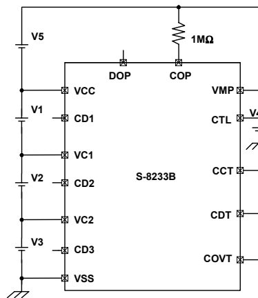
Measurement circuit 10
