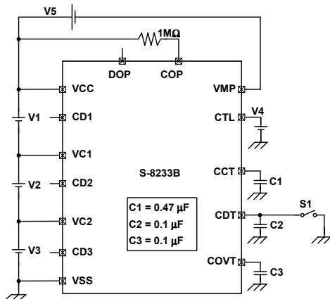
Measurement circuit 7
