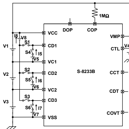
Measurement circuit 8
