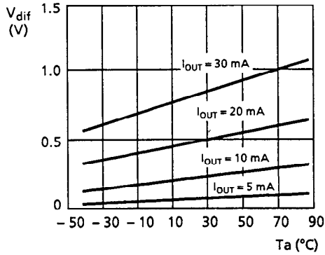
7.9 S-81250SG series
