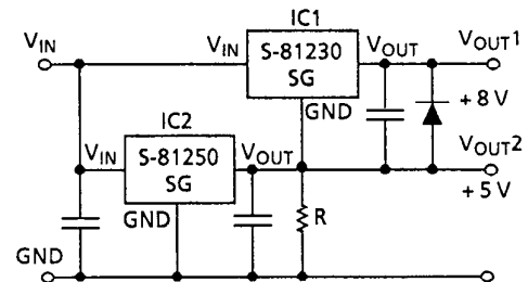
Figure 17 Dual power source
