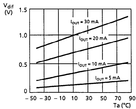
7.5 S-81230SG series
