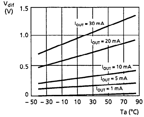
7.4 S-81225SG series
