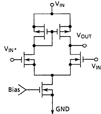
Figure 5 Error amplifier
