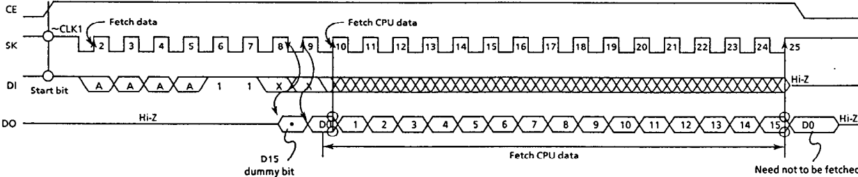
Figure 13 Read mode timing(S-24H45, S-24S45)
