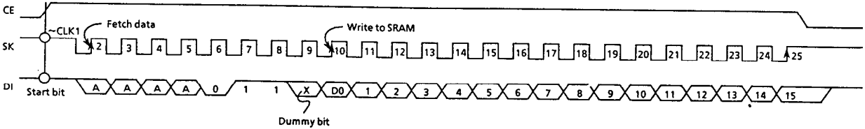
Figure 15 Write mode timing(S-24H45, S-24S45)
