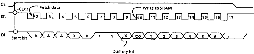
Figure 16 Write mode timing(S-24H30, S-24S30)
