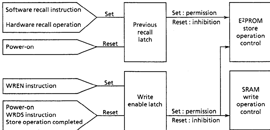
Figure 7 Internal latch
