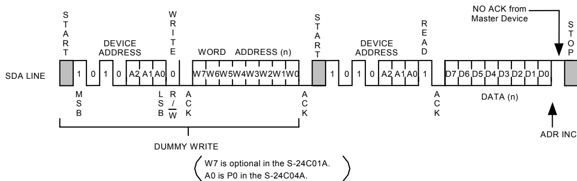
Figure 13 Random Read
