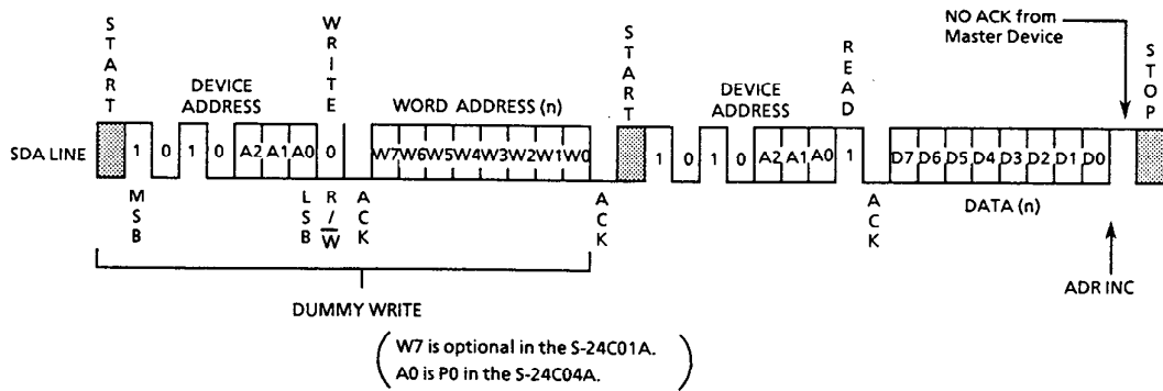
Figure 13 Random Read
