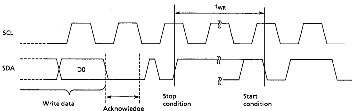
Figure 5 Write Cycle
