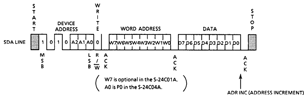
Figure 10 Byte Write
