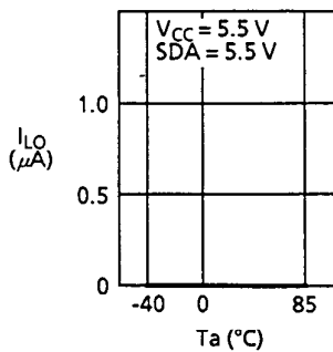
1.15 Output leakage current I_{LO} - Ambient temperature T_a
