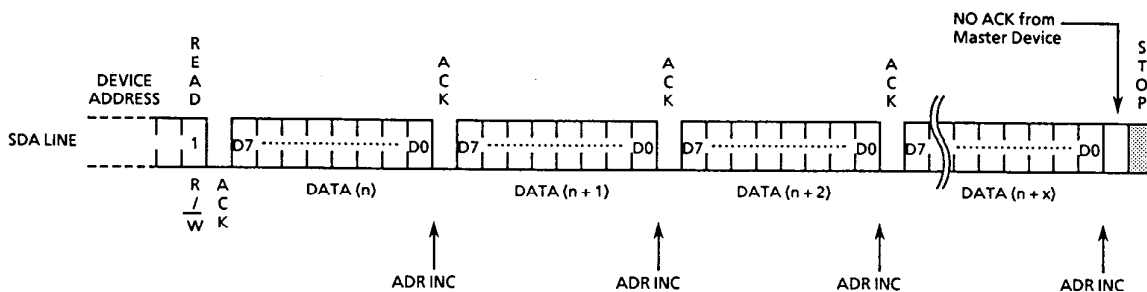
Figure 14 Sequential Read
