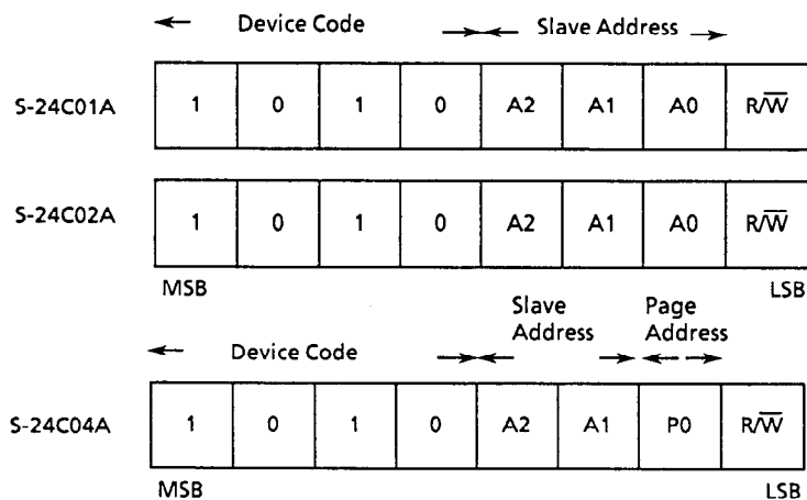
Figure 9 Device Address
