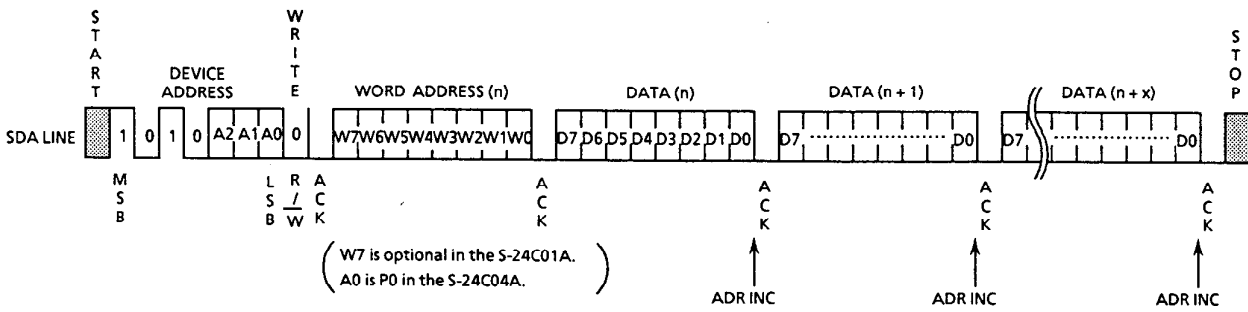
Figure 11 Page Write
