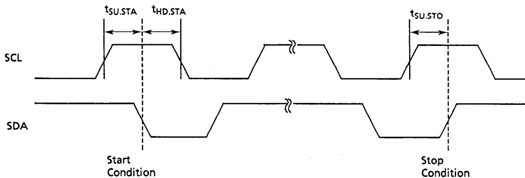
Figure 6 Start/Stop Conditions
