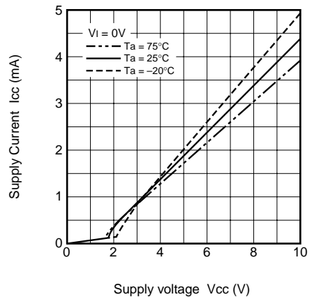
Driver Supply Characteristics
