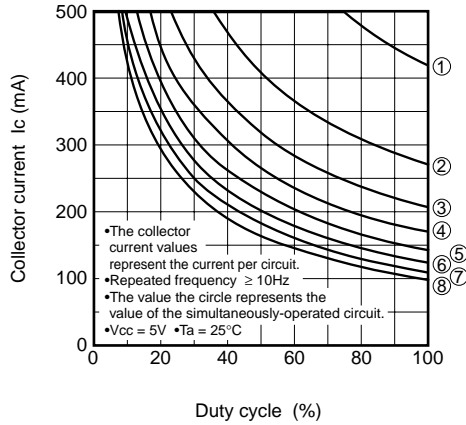
Duty Cycle-Collector Characteristics (M54587FP)
