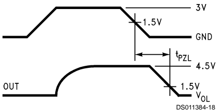
FIGURE 16. Receiver Enable and Disable Timing
