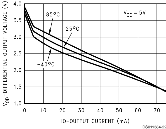
Differential Output Voltage vs Output Current
