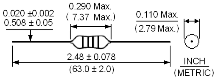
Mechanical drawing
