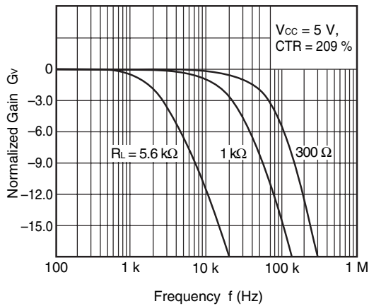
FREQUENCY RESPONSE
