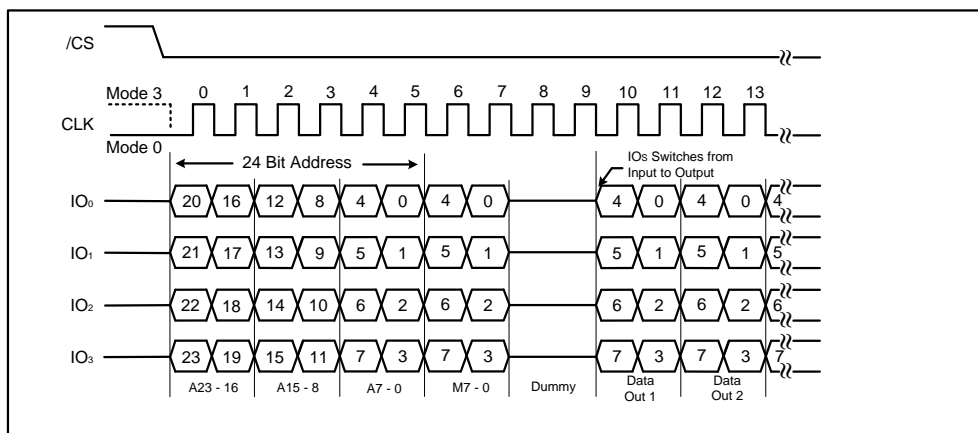
Figure 35b. Word Read Quad I/O instruction (Previous instruction set M7-0= Ahx, SPI Mode)
