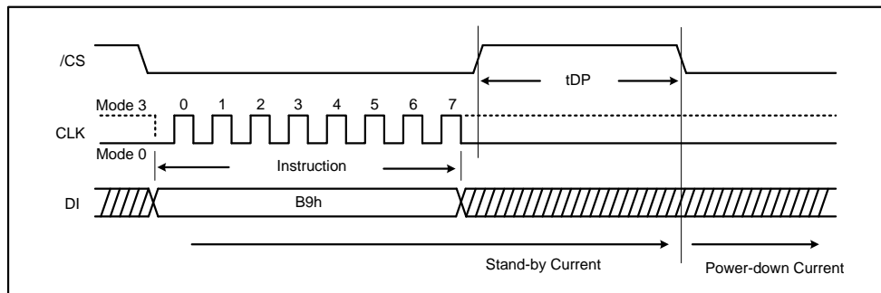
Figure 27a. Deep Power-down Instruction (SPI Mode)
