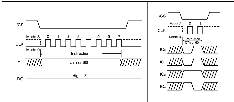
Figure 24. Chip Erase Instruction for SPI Mode (left) and QPI Mode (right)
