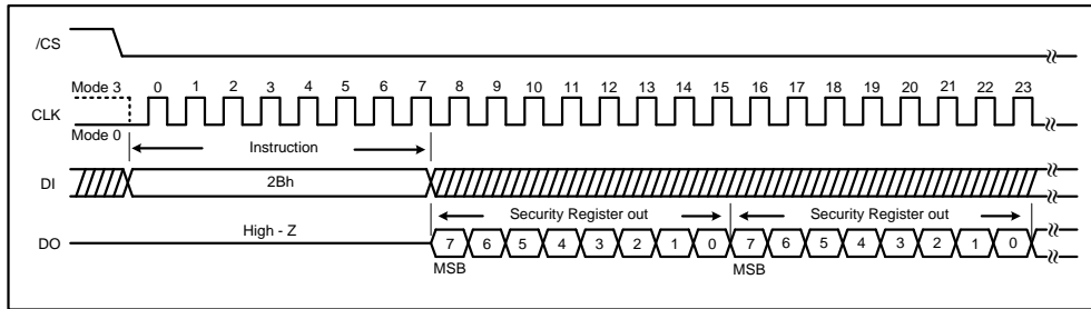
Figure 43a. Read Security Register instruction (SPI Mode)
