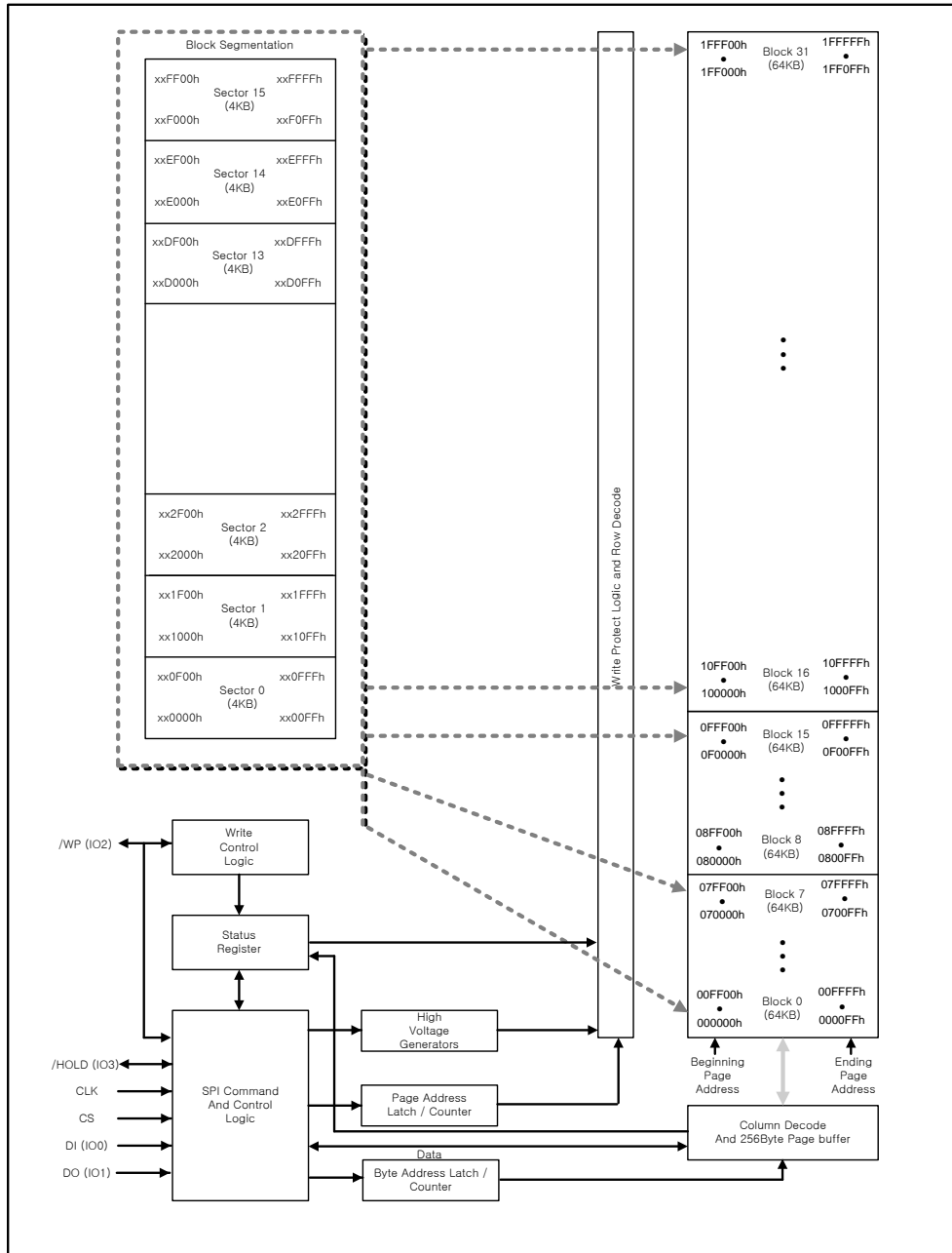
Figure 2. Block Diagram of FM25M16A
