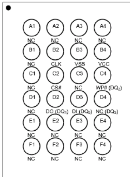
24 - Ball TFBGA
