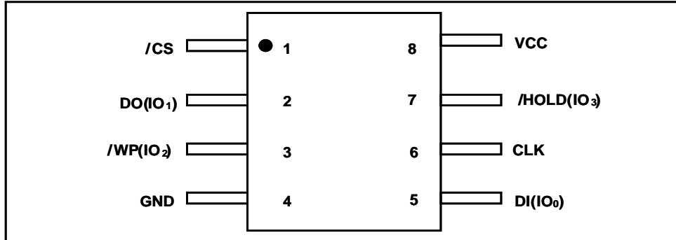
Figure 1a. Pin Assignments, 8-pin SOIC 150-mil / 208-mil / VSOP 208-mil
