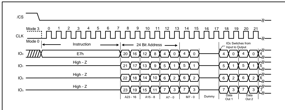
Figure 35a. Word Read Quad I/O instruction (Initial instruction or previous set M7-0 ≠ Ahx, SPI Mode)
