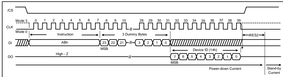
Figure 28c. Release power-down / Device ID Instruction (SPI Mode)
