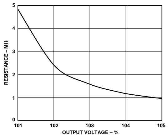
Figure 31. External Resistor for Increasing Output Voltage
