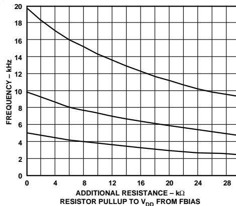
Figure 2. Typical Added Resistance Value
