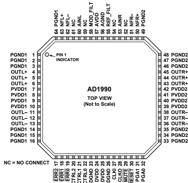
Figure 3. Pin Configuration
