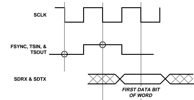
Figure 6. AD1849K Timing Relationships
