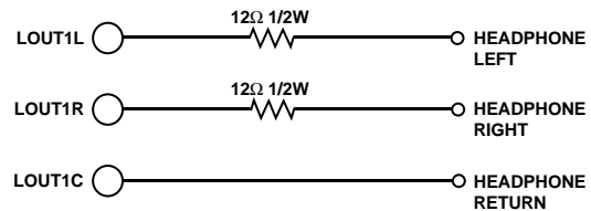
Figure 15. AD1849K Optional Headphone Drive Connections
