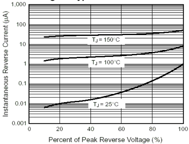
Fig. 3 – Typical Reverse Current
