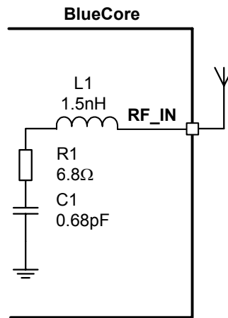
Figure 10.2: Circuit RF_IN
