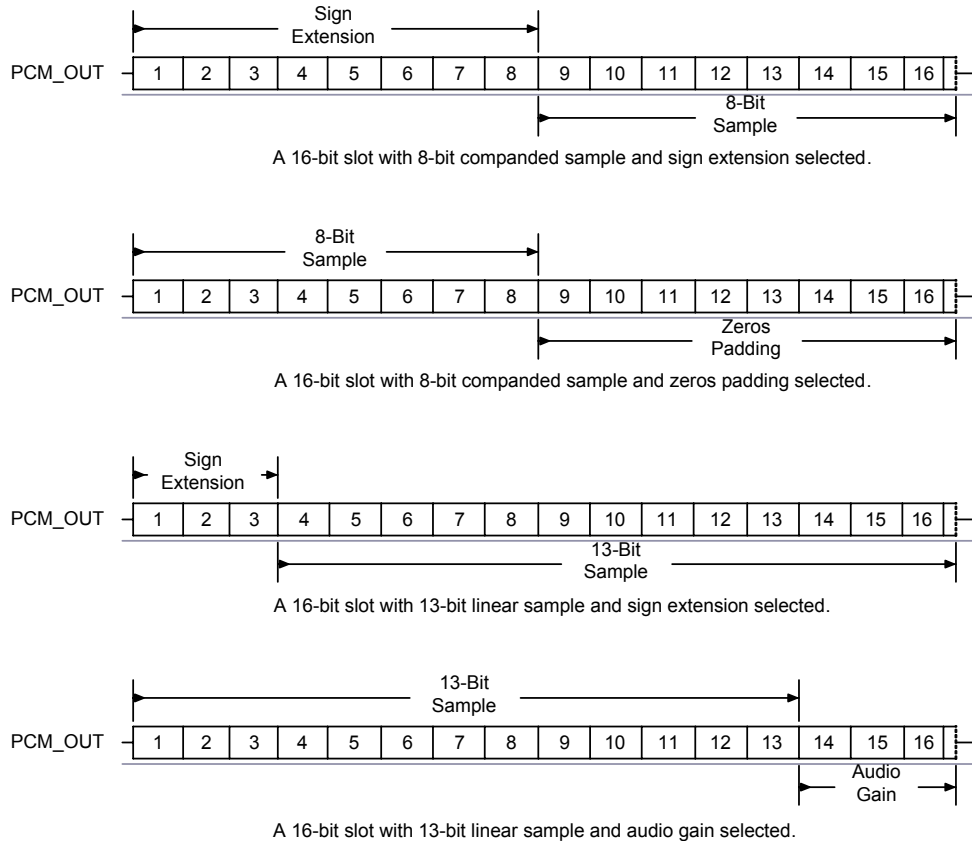
Figure 10.24: 16-Bit Slot Length and Sample Formats
