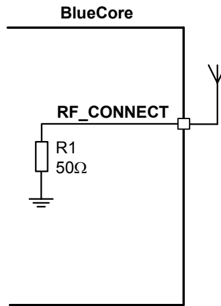
Figure 10.1: Circuit for RF_CONNECT
