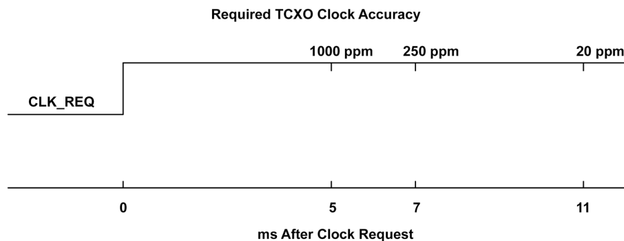
Figure 10.3: TCXO Clock Accuracy
