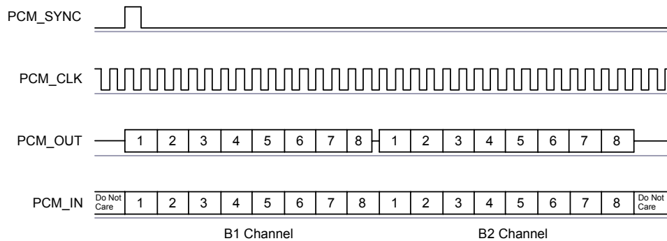
Figure 10.23: GCI Interface
