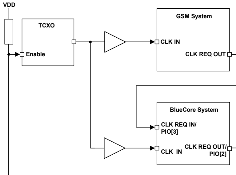
Figure 10.30: Example TXCO Enable OR Function
