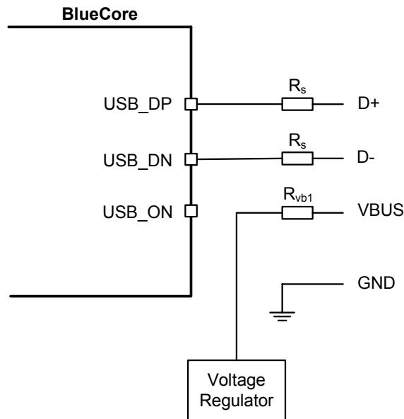
Figure 10.14: USB Connections for Bus-Powered Mode
