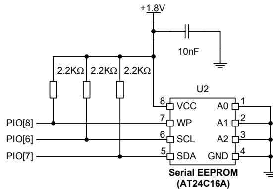
Figure 10.29: Example EEPROM Connection
