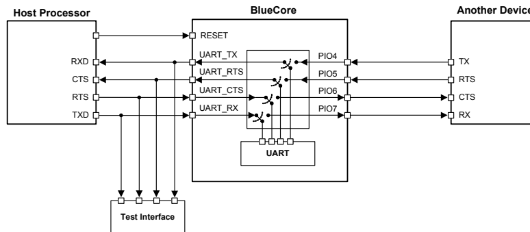
Figure 10.12: UART Bypass Architecture
