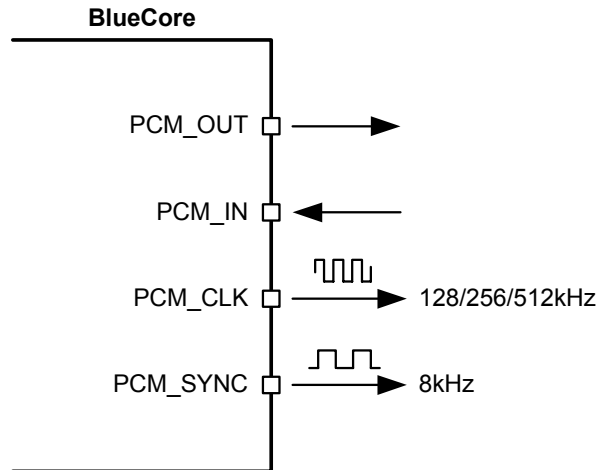
Figure 10.18: BlueCore4-ROM Plug-n-Go as PCM Interface Master
