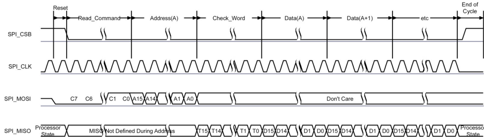
Figure 10.17: Read Operation
