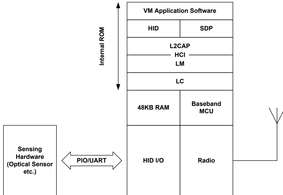
Figure 9.4: HID Stack
