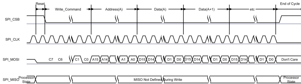
Figure 10.16: Write Operation
