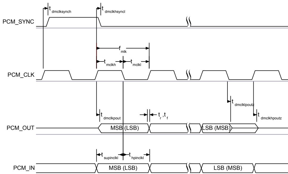
Figure 10.26: PCM Master Timing Short Frame Sync
