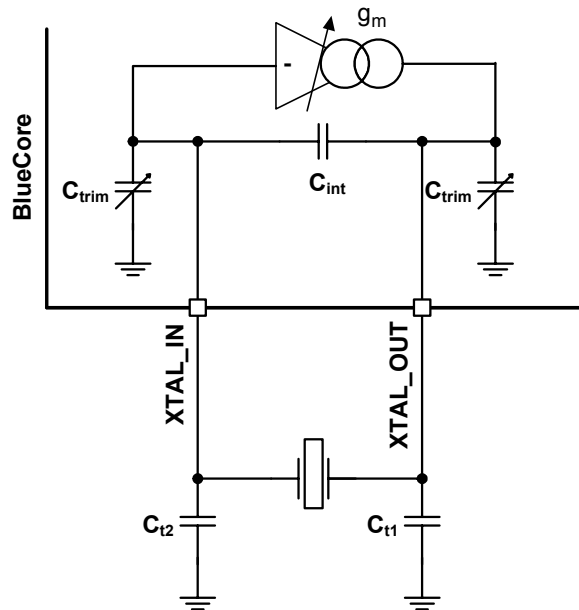
Figure 10.5: Crystal Driver Circuit
