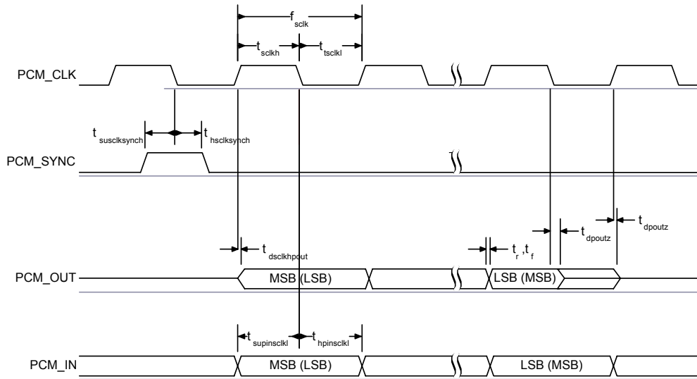
Figure 10.28: PCM Slave Timing Short Frame Sync
